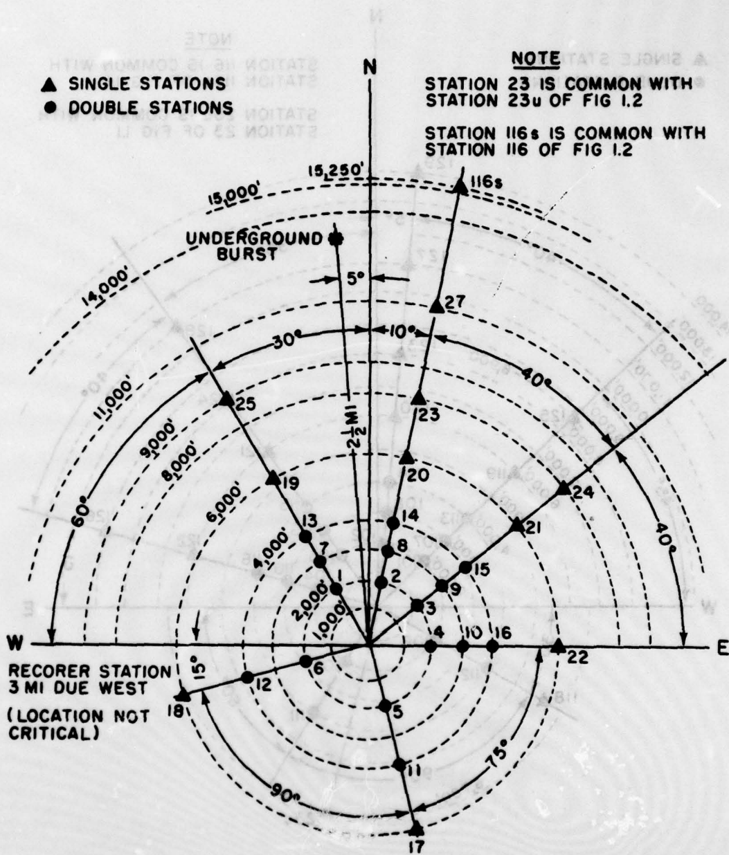
Fig. A.3 Station Pattern of Surface Burst for Project 2. 1a (Fig. 1.1, WT-370)
